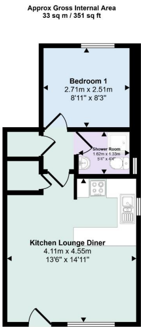
Floorplan
